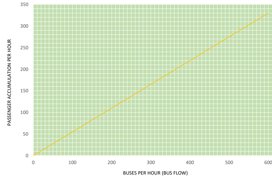
Passenger Accumulation
