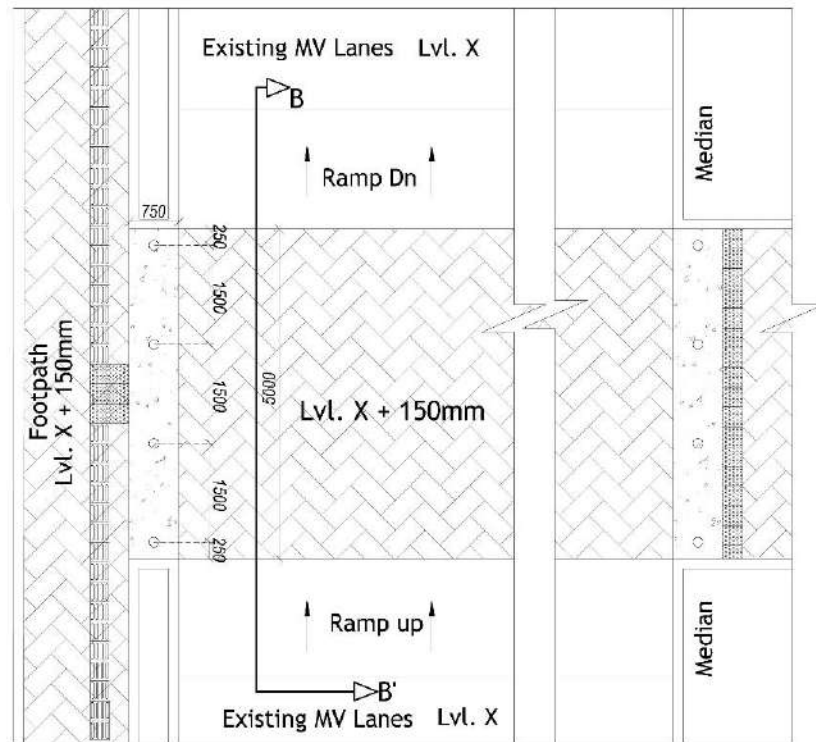
PLAN
