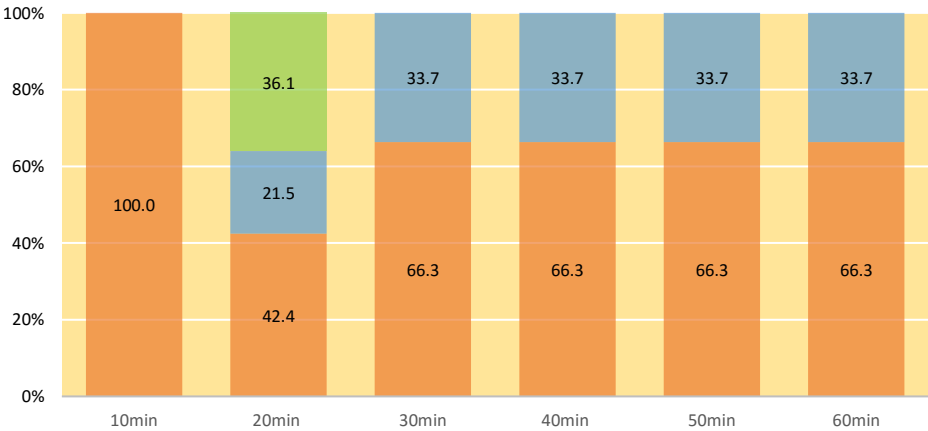
Large Terminals
